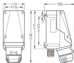
16A 4P 壁式插座 Wall socket 4-pole
