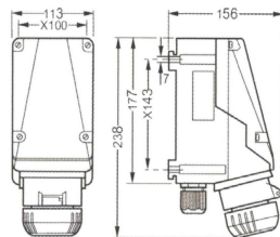
16A 4P 壁式插座 Wall socket 4-pole
